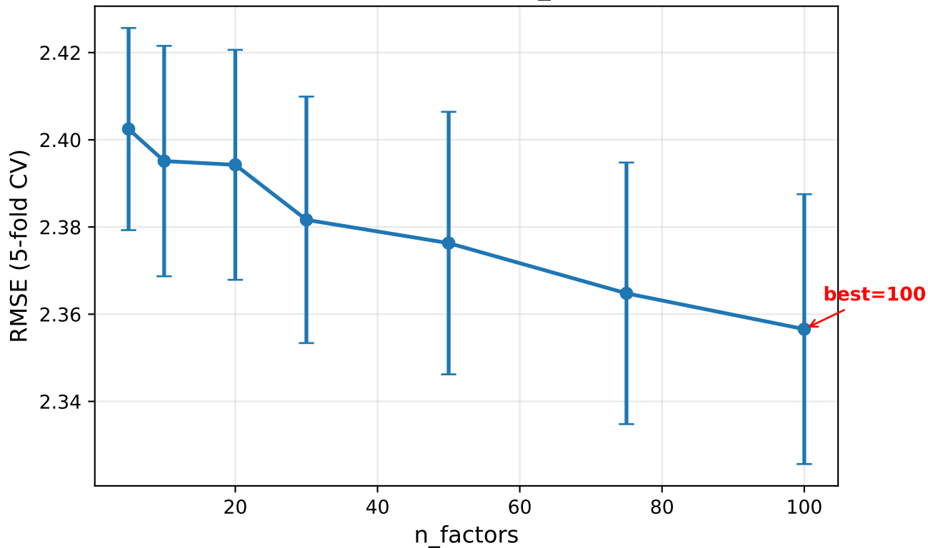
Sensitivity: bpr — n_factors
