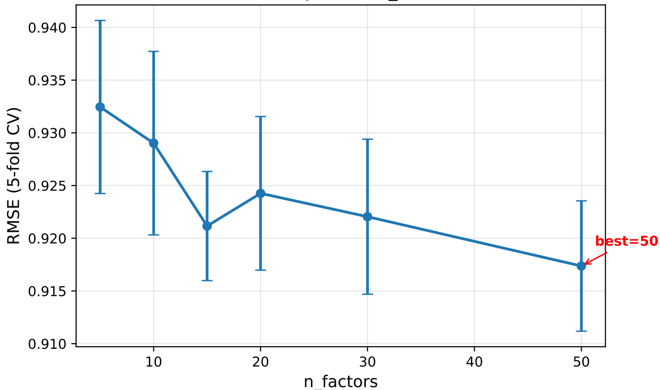
Sensitivity: fm — n_factors
