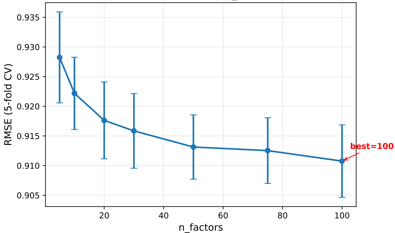
Sensitivity: svd — n_factors
