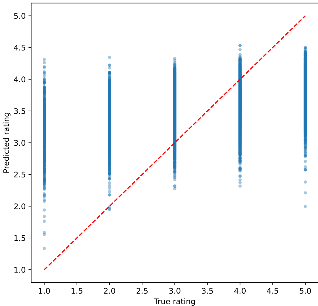
Scatter: RMSE=0.995, MAE=0.804
