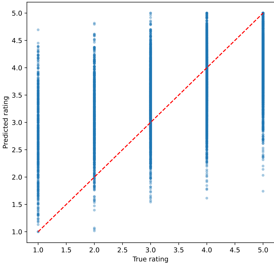
Scatter: RMSE=0.933, MAE=0.734
