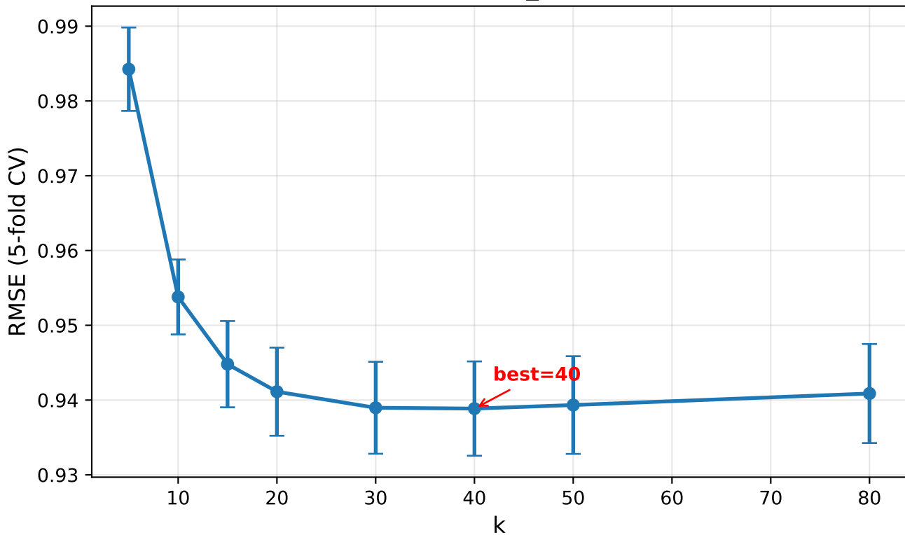
Sensitivity: user_based — k
