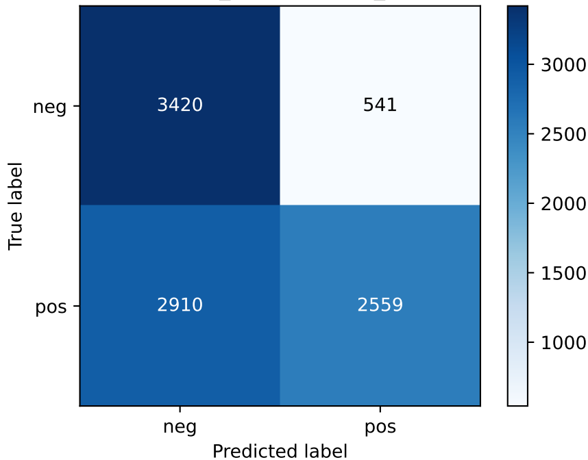
Confusion (thr_true=4.0, thr_pred=4.0)
