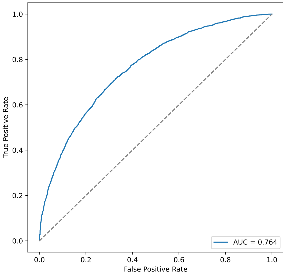
ROC (threshold=4.0)
