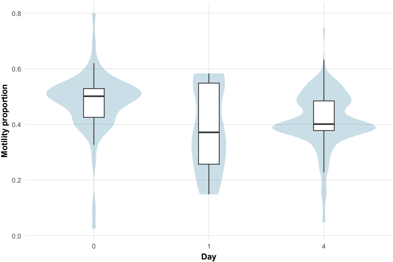
Distribution of motility fractions at key days
