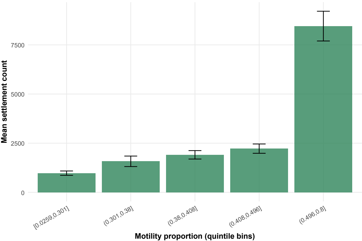
Settlement increases with motility (binned means \pm SE)
