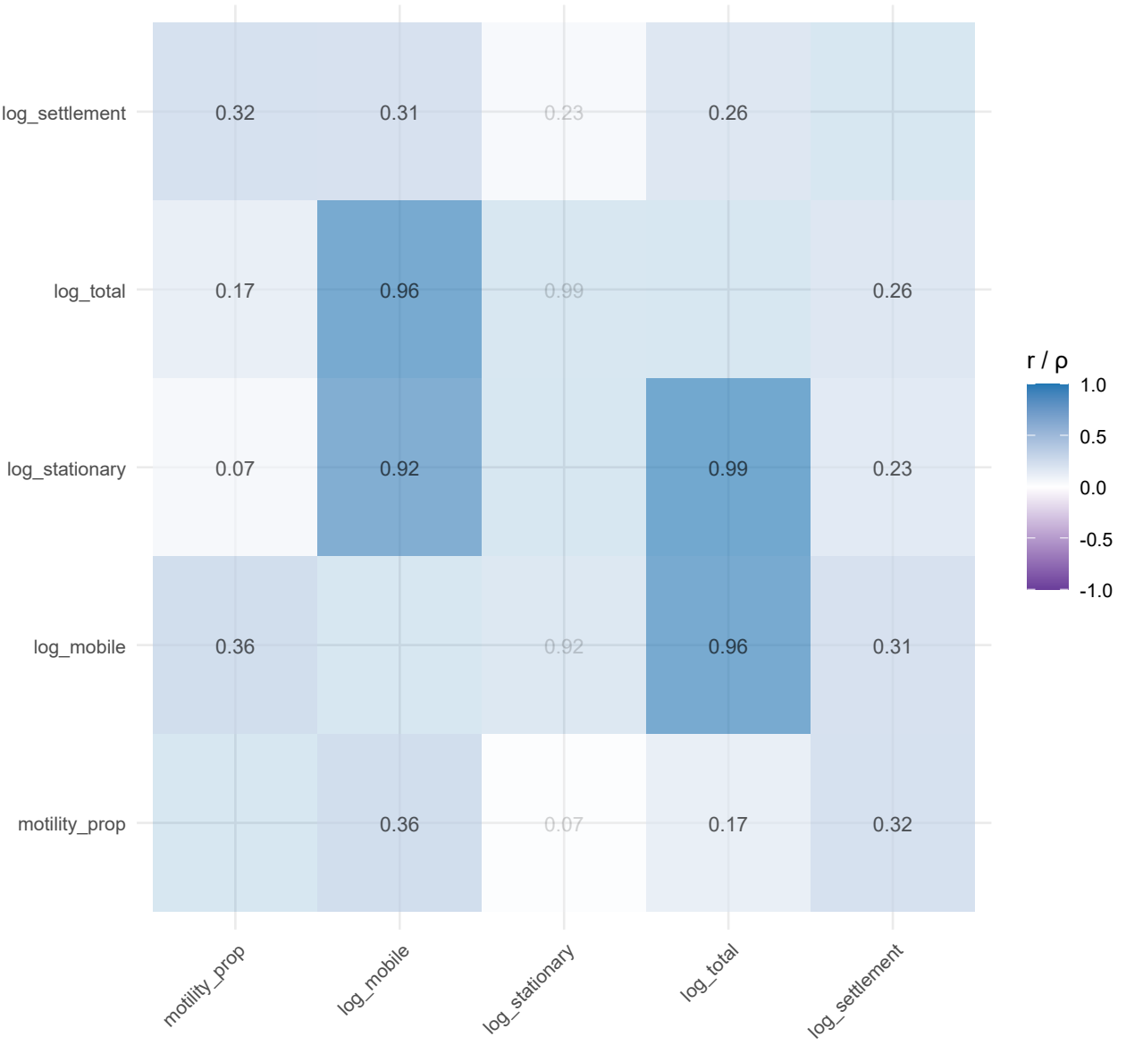
Correlations — day4 (spearman) Cells dimmed when q \geq 0.05 ; '*' marks n < 15
