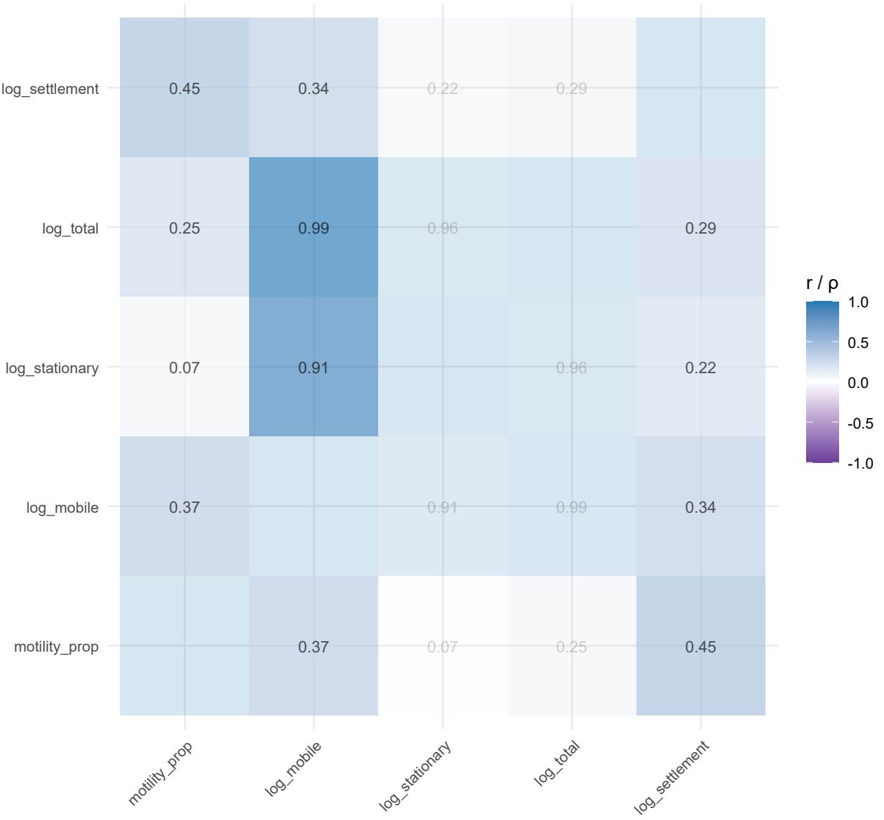
Correlations — day0 (spearman) Cells dimmed when q \geq 0.05 ; '*' marks n < 15
