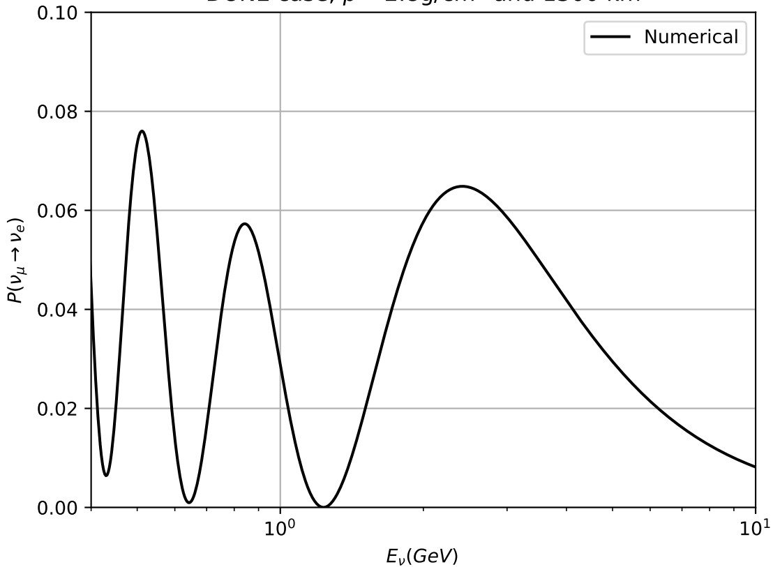
DUNE case, \rho = 2.8\text{g/cm}^3 and 1300 km
