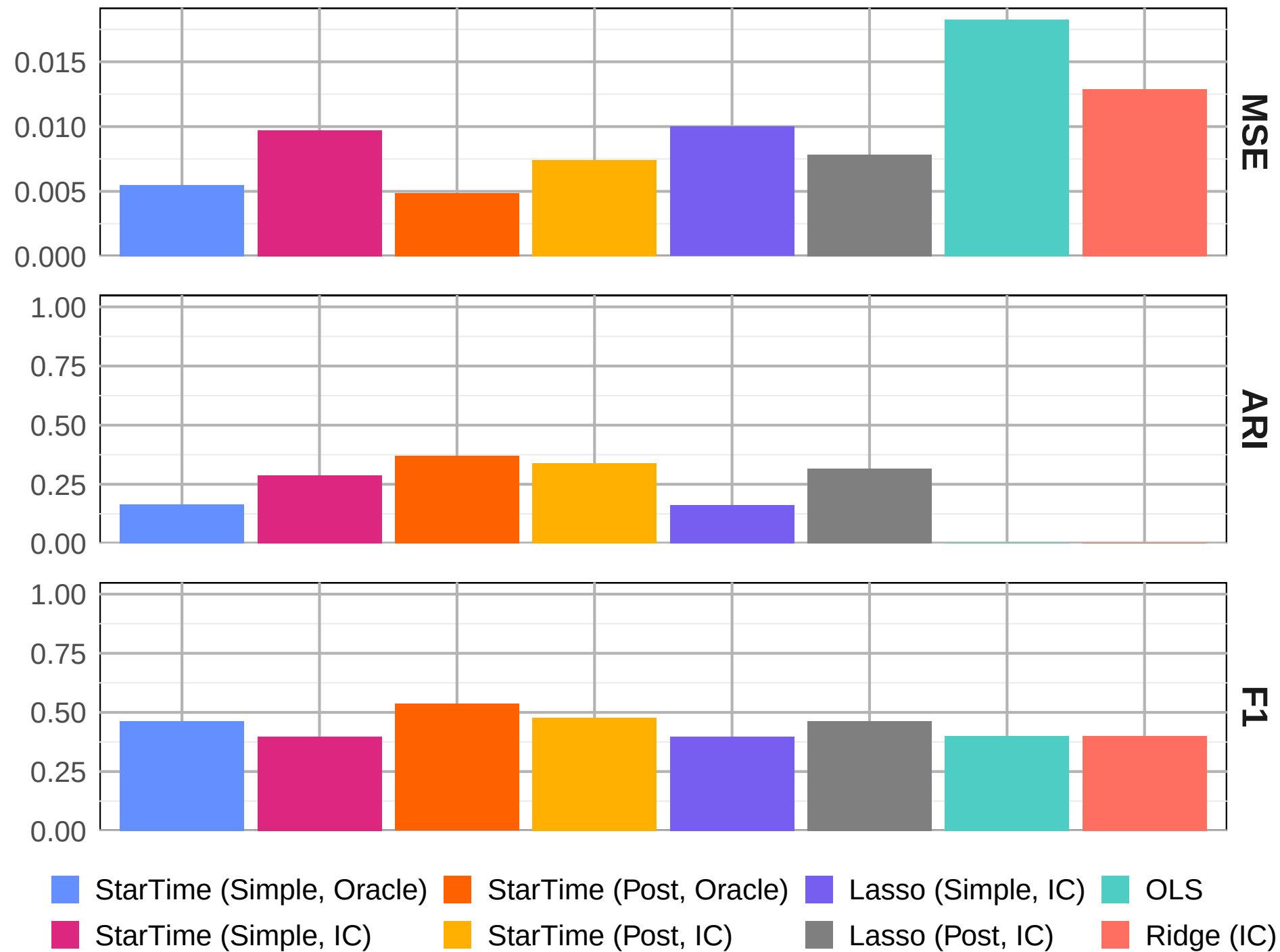
AR DGP 3, T = 100
