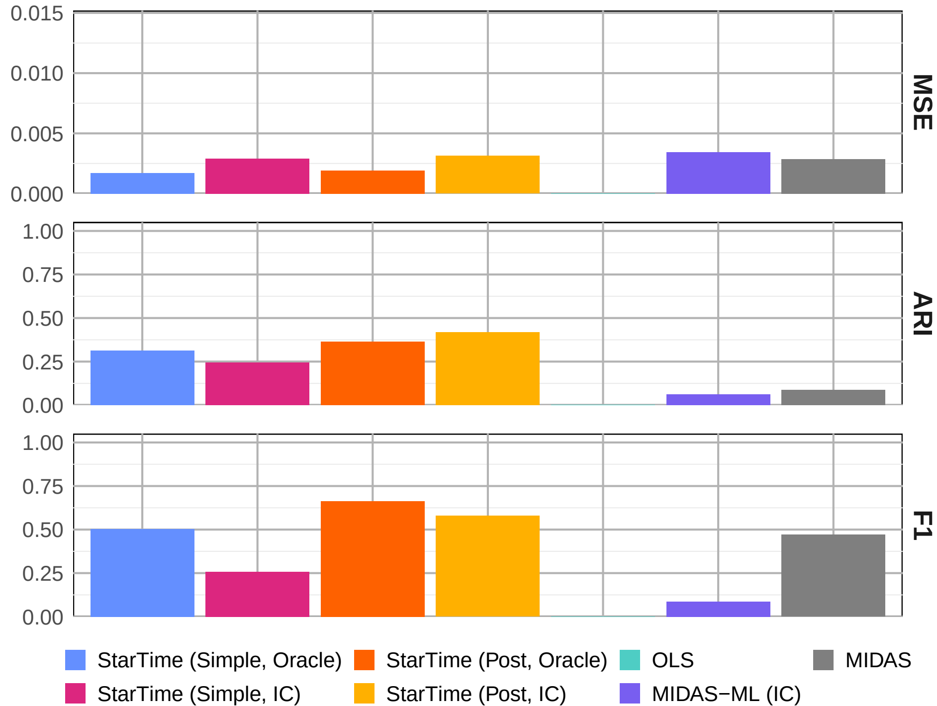
Mixed DGP 2, T = 100
