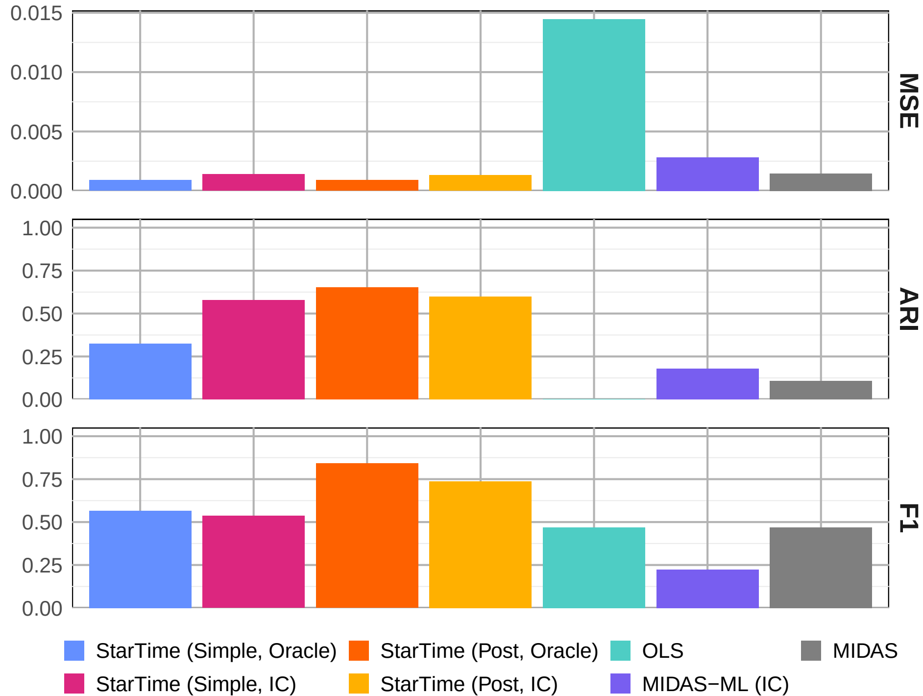
Mixed DGP 2, T = 200
