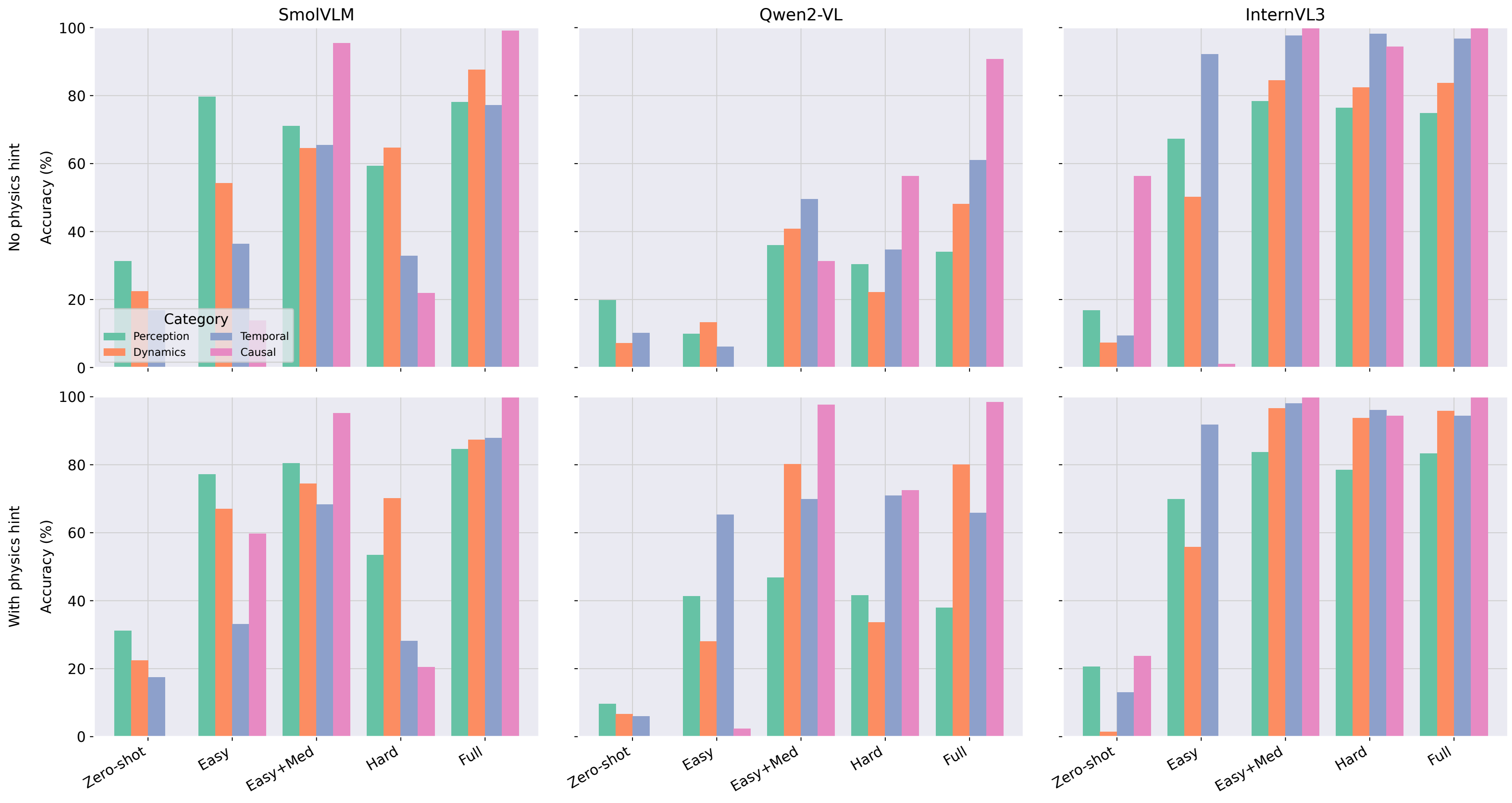
Capability profile: accuracy by reasoning category
