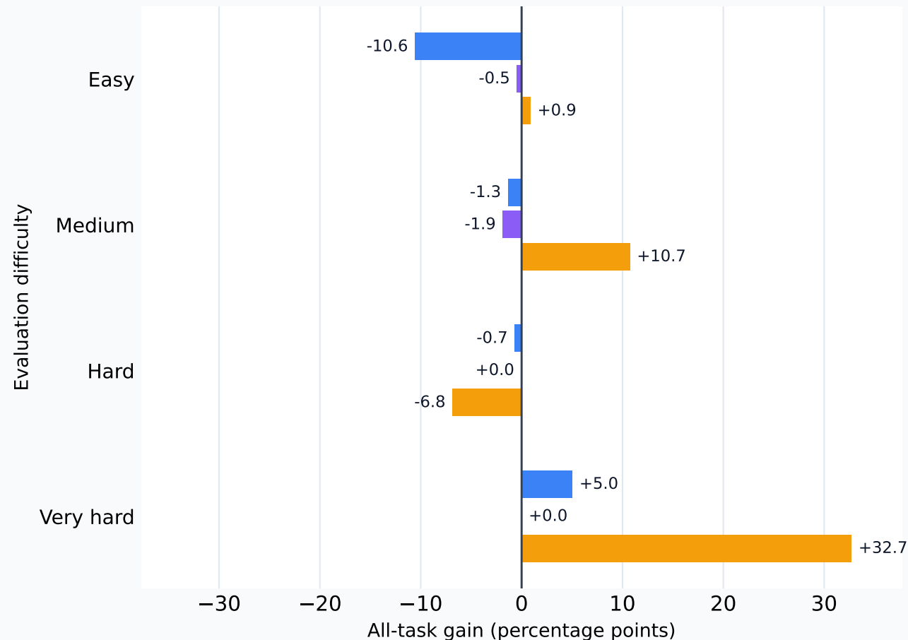
Physics augmented
