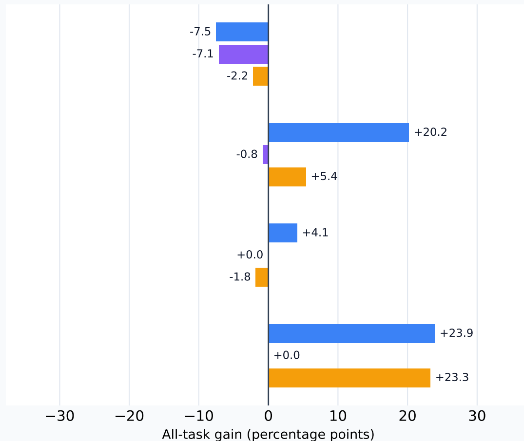
No physics
