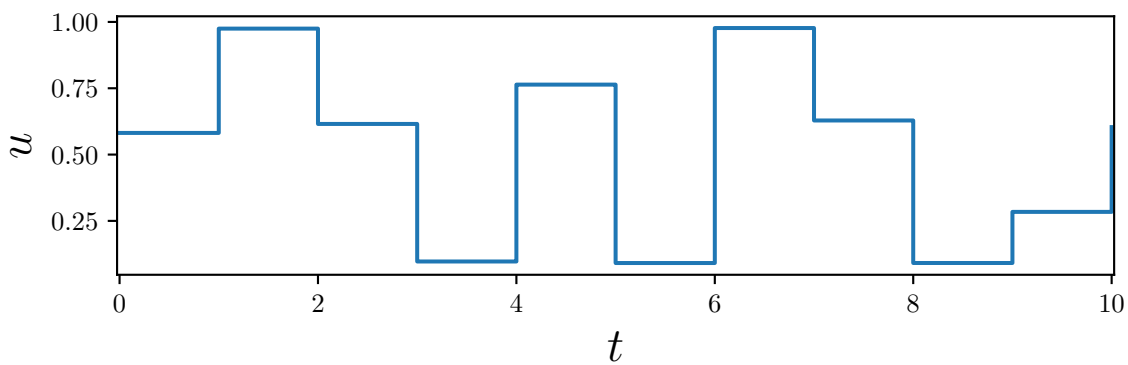
\theta = (0.20, 0.25)
