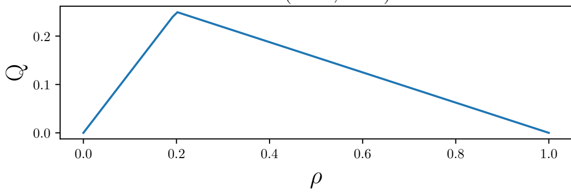
\theta = (0.20, 0.25)
