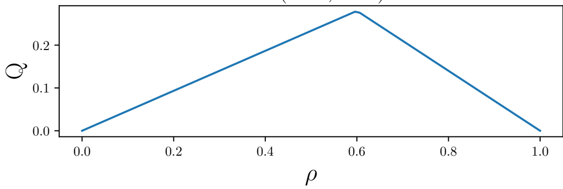
\theta = (0.60, 0.28)
