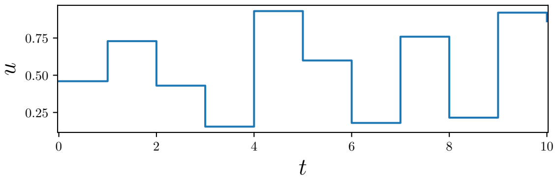
\theta = (0.60, 0.28)
