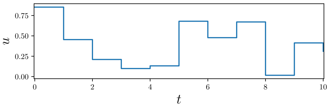
\theta = (0.80, 0.29)
