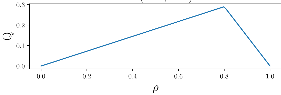
\theta = (0.80, 0.29)
