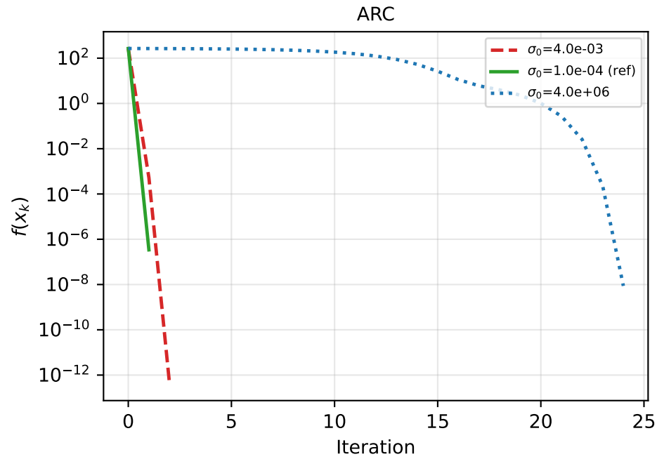
Quadratic \kappa=1e2 — convergence by \sigma_0
