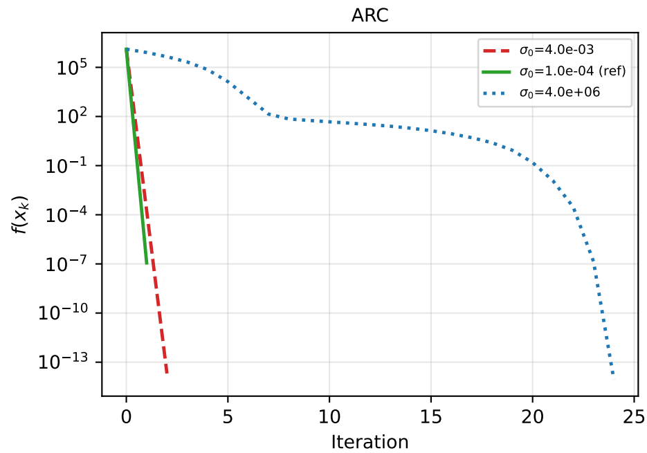
Quadratic \kappa=1e6 — convergence by \sigma_0
