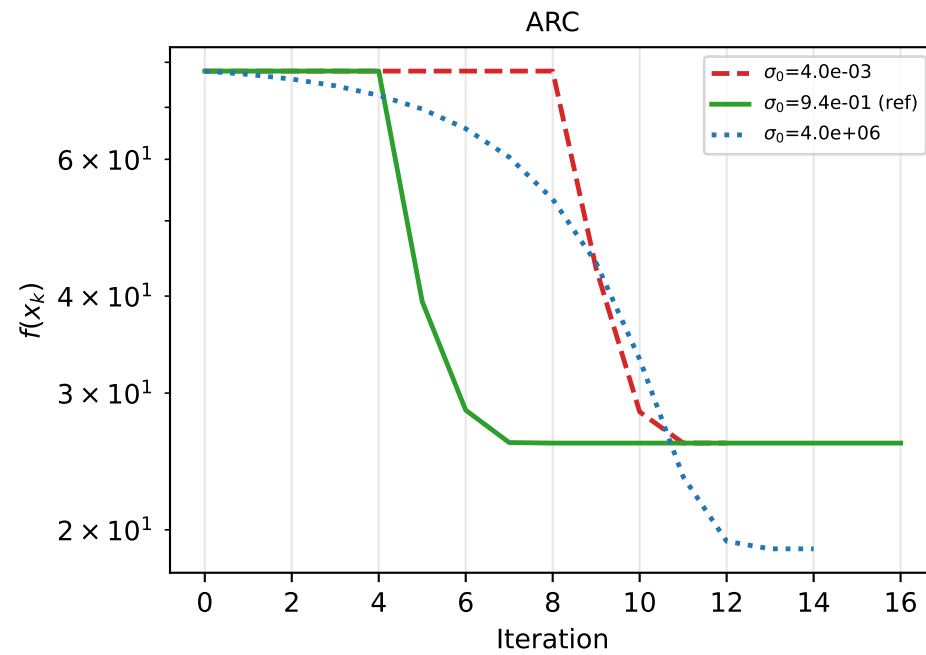
Rastrigin n=10 — convergence by \sigma_0
