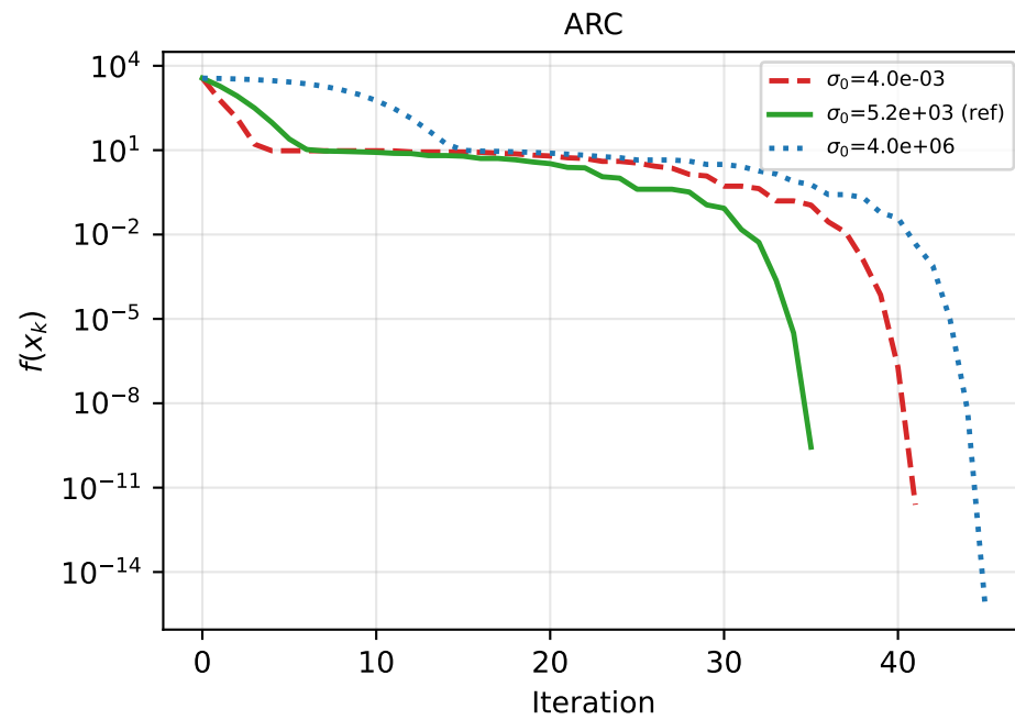
Rosenbrock n=10 — convergence by \sigma_0
