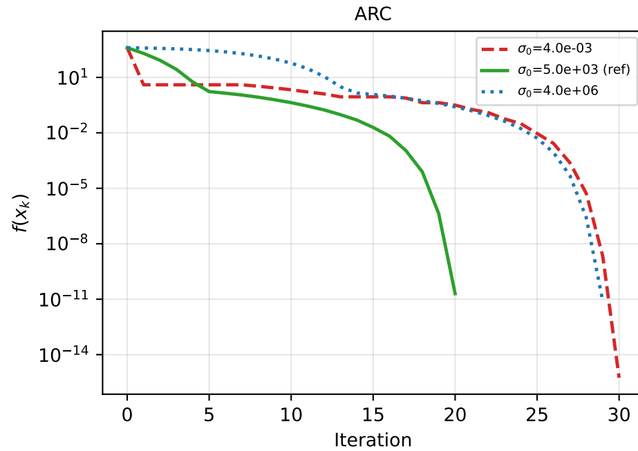
Rosenbrock n=2 — convergence by \sigma_0
