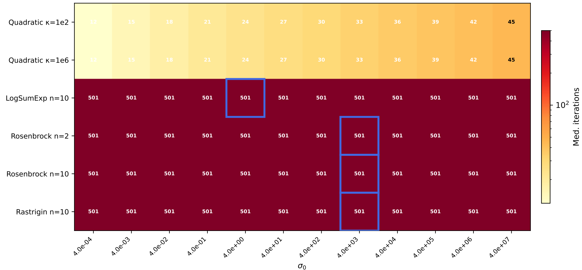
ACRN — Median iterations (blue = \sigma_{\text{ref}} )
