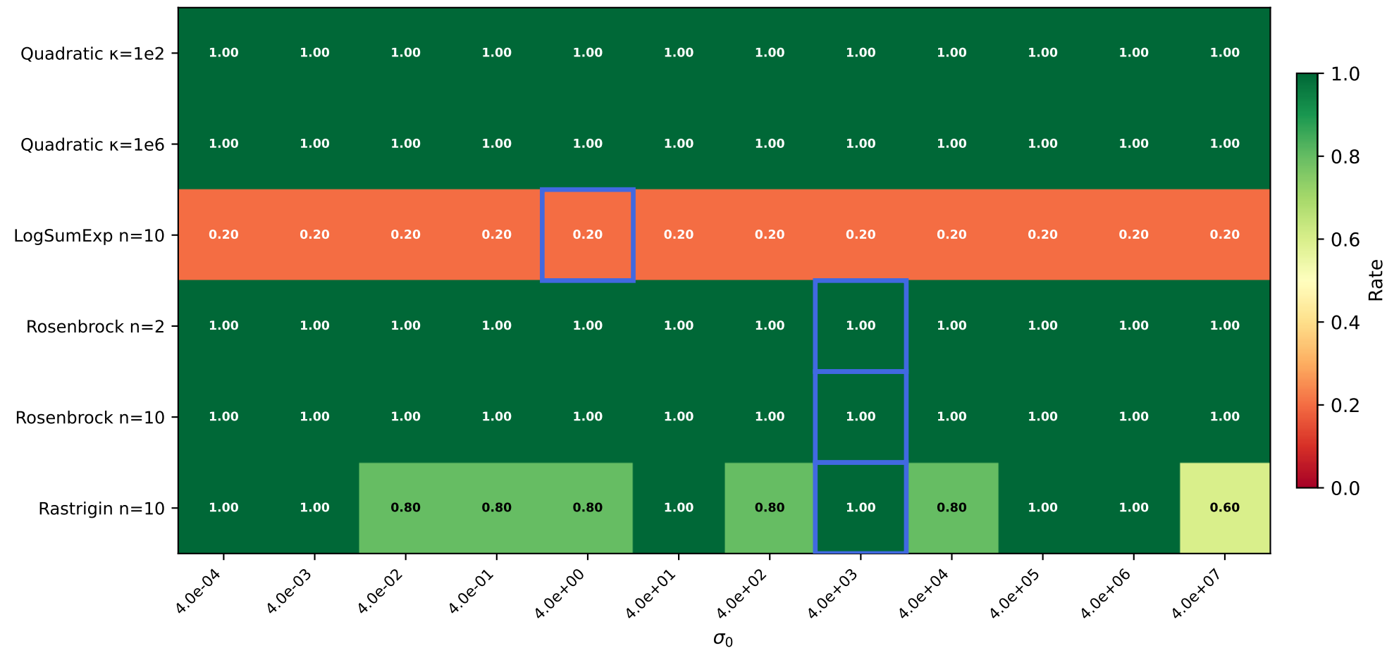
ARC — Success rate ( \text{blue} = \sigma_{\text{ref}} )
