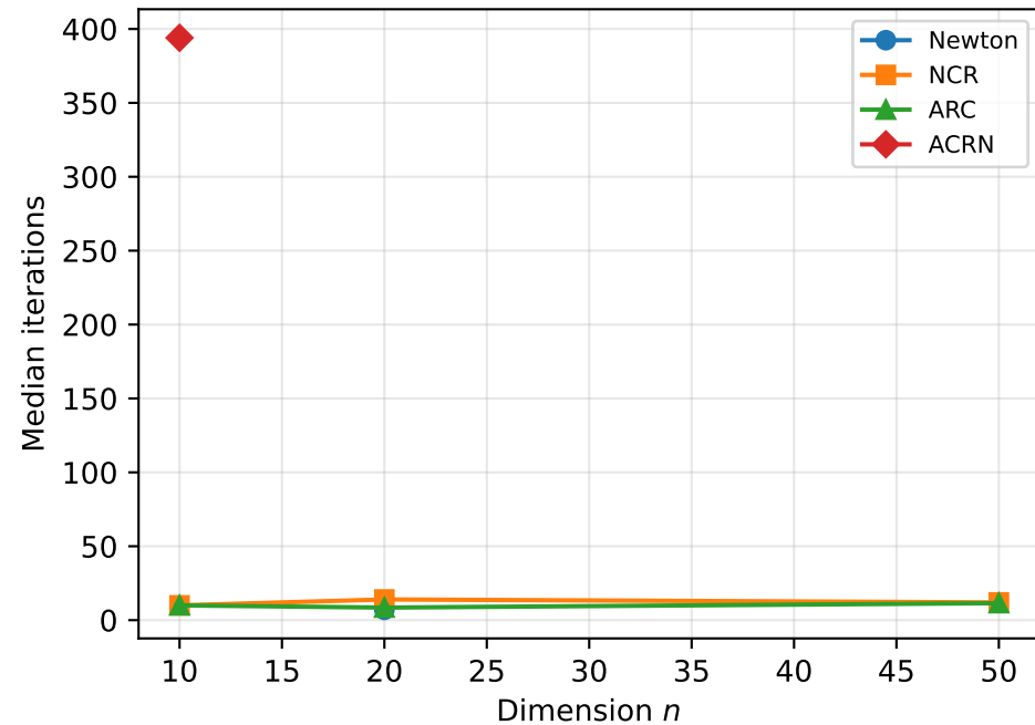
Logsumexp
