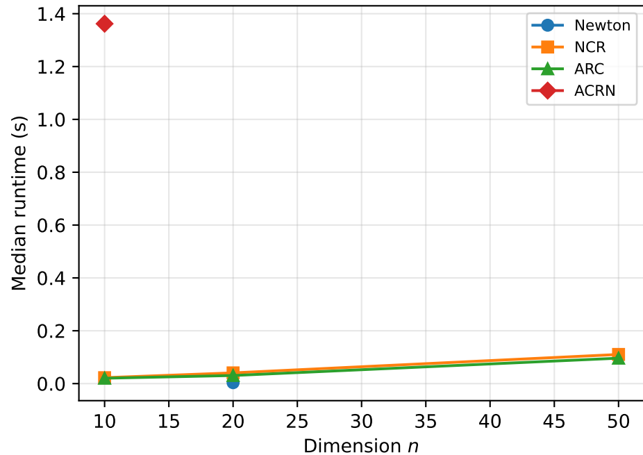
Logsumexp
