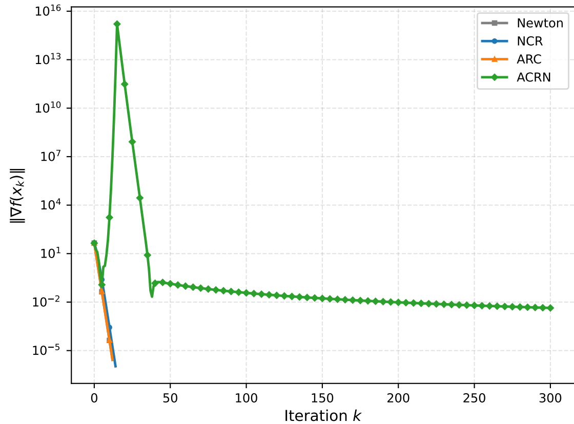
Cubic norm (n=10) Gradient norm
