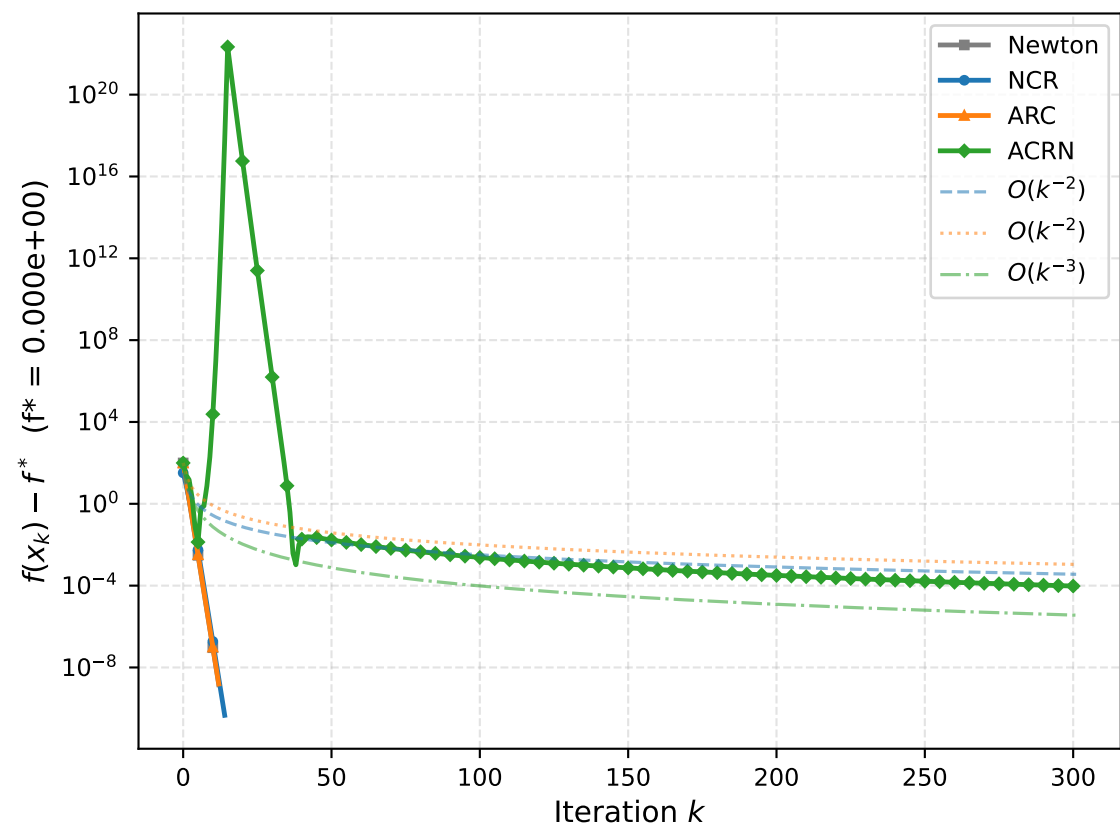
Cubic norm (n=10) Function excess
