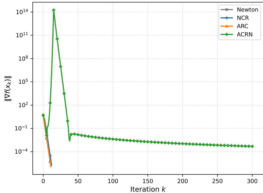
Cubic norm (n=2) Gradient norm
