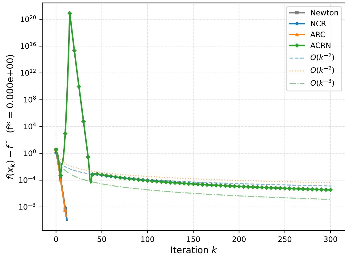
Cubic norm (n=2) Function excess
