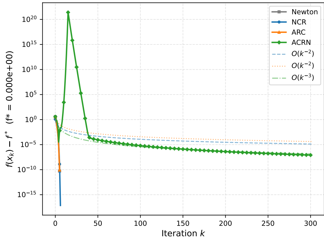
Cubic poly (n=2, \gamma=1 ) Function excess
