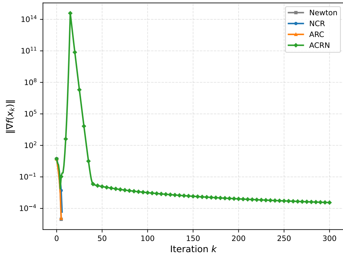
Cubic poly (n=2, \gamma=1 ) Gradient norm
