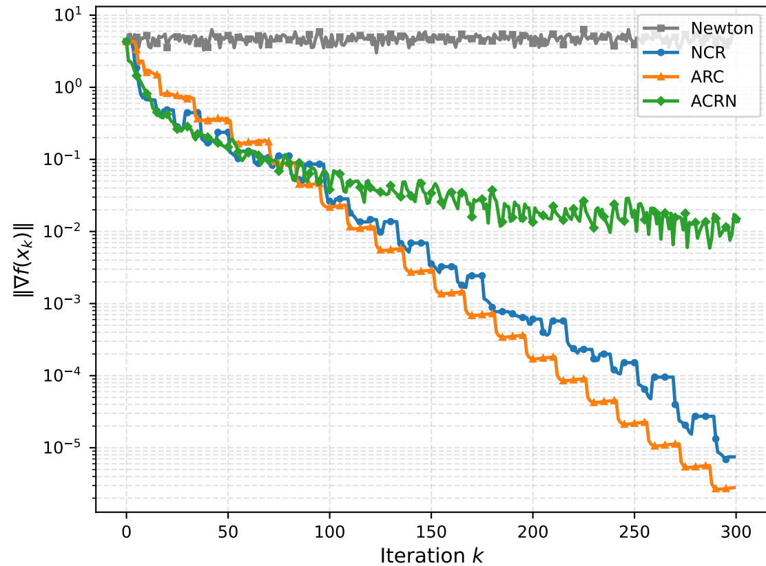
LogSumExp ( n=20, \mu=0.2 ) Gradient norm
