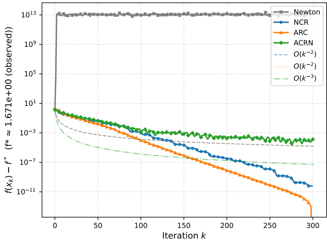
LogSumExp ( n=20, \mu=0.2 ) Function excess
