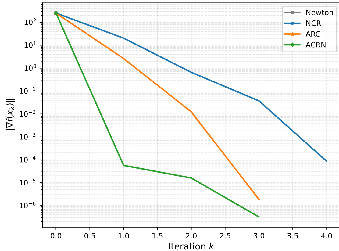
Quadratic ( n=5 , \kappa=1e+02 ) Gradient norm
