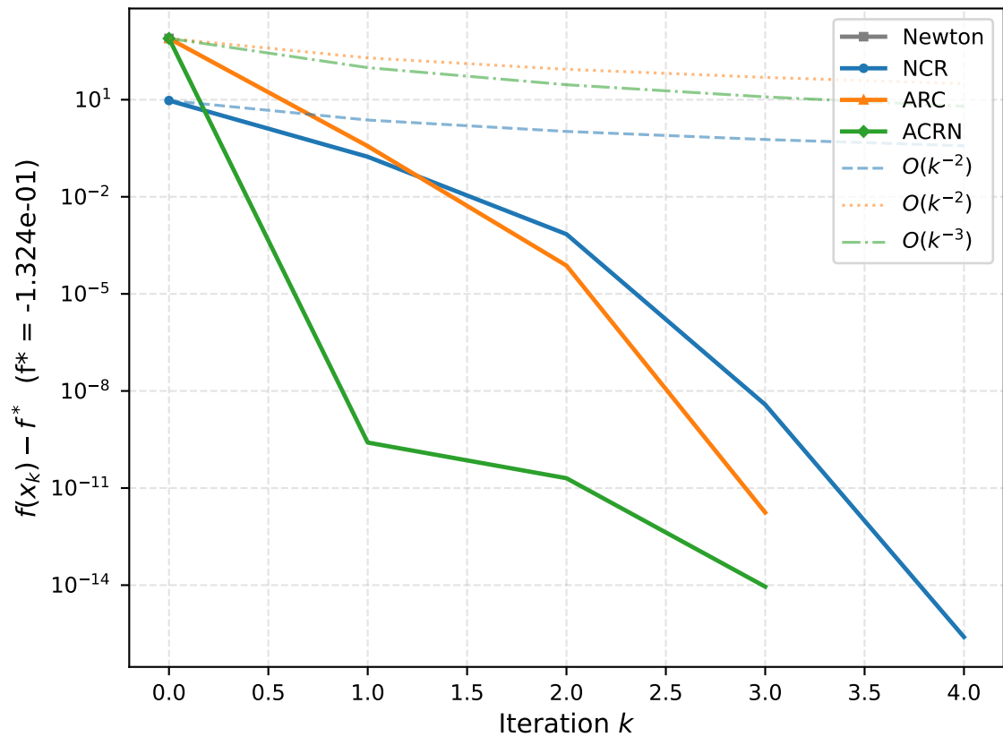
Quadratic ( n=5 , \kappa=1e+02 ) Function excess
