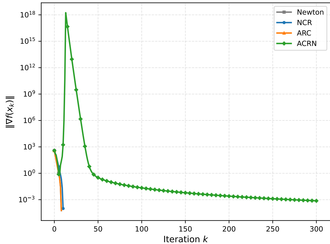
Quartic convex (n=10) Gradient norm
