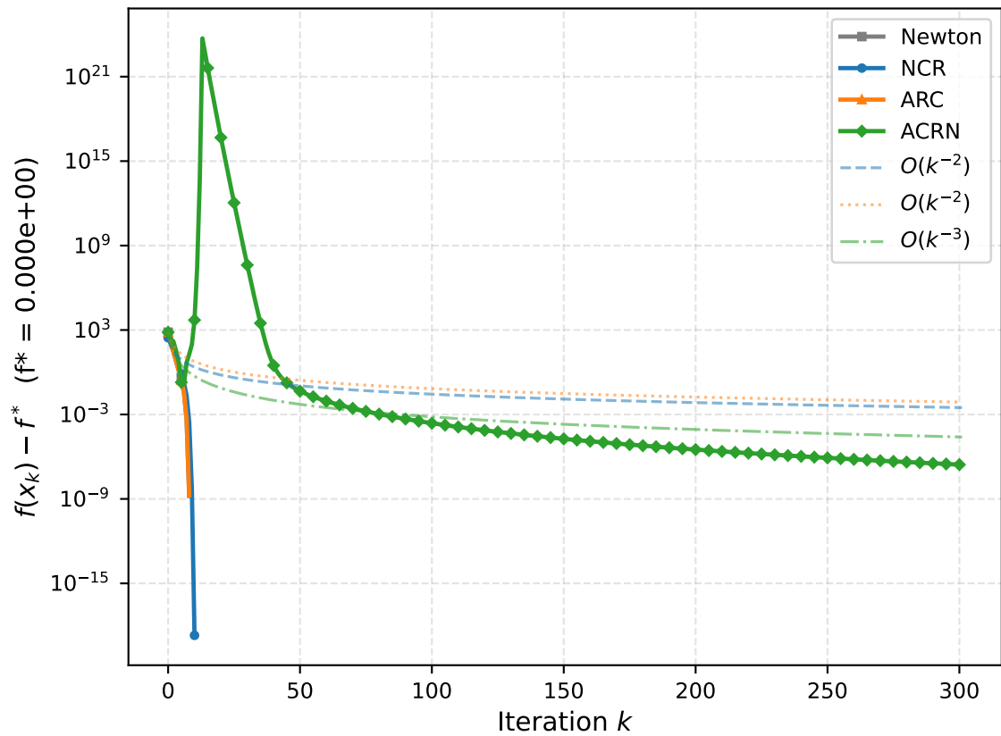
Quartic convex (n=10) Function excess
