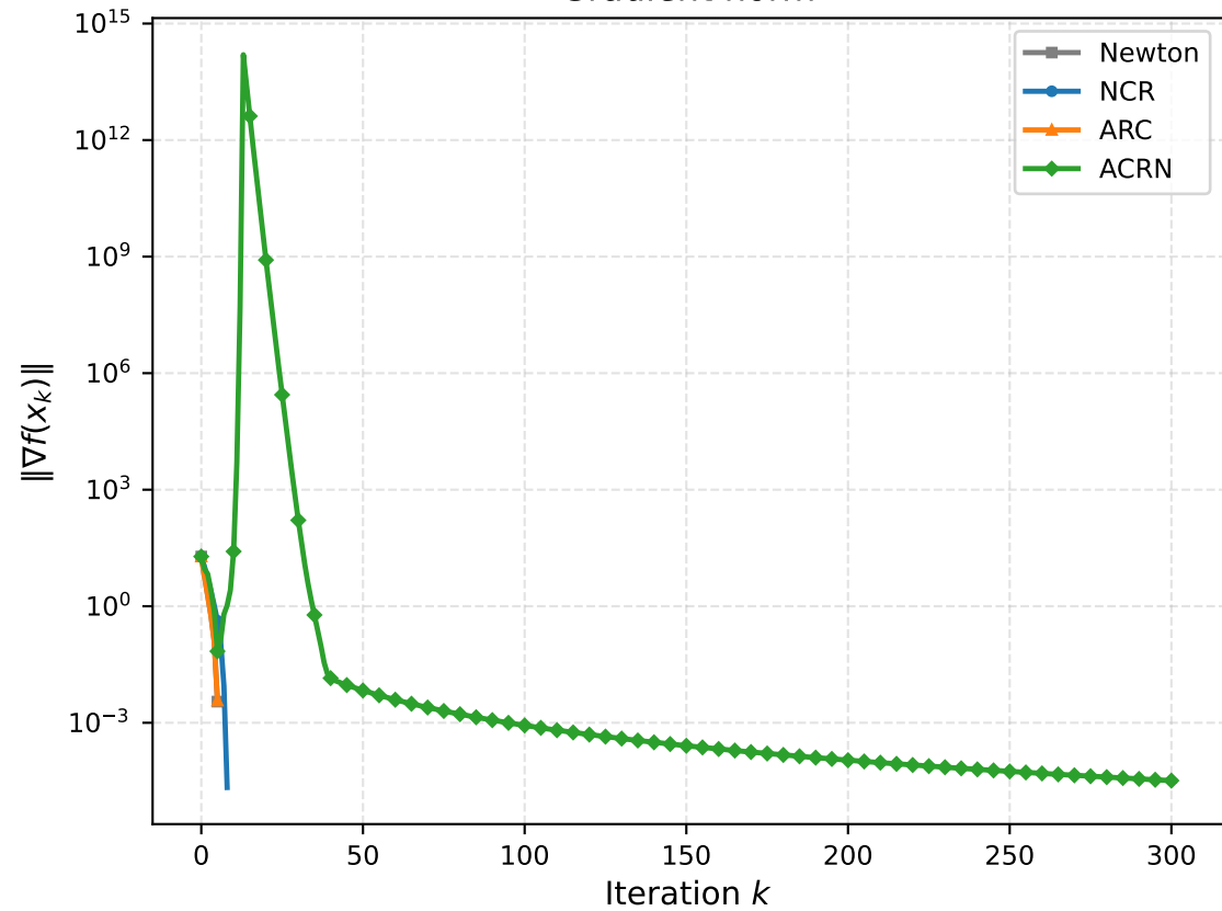
Quartic convex (n=2) Gradient norm
