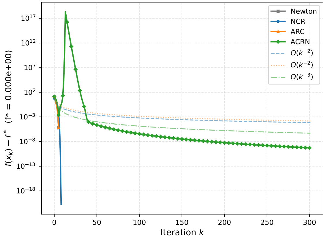
Quartic convex (n=2) Function excess
