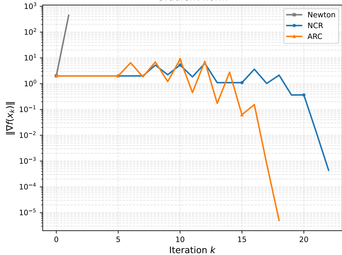
Rosenbrock (n=2) Gradient norm
