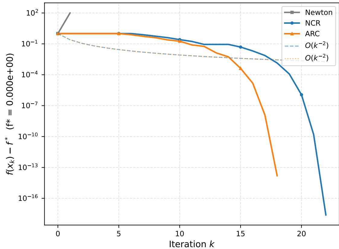
Rosenbrock (n=2) Function excess
