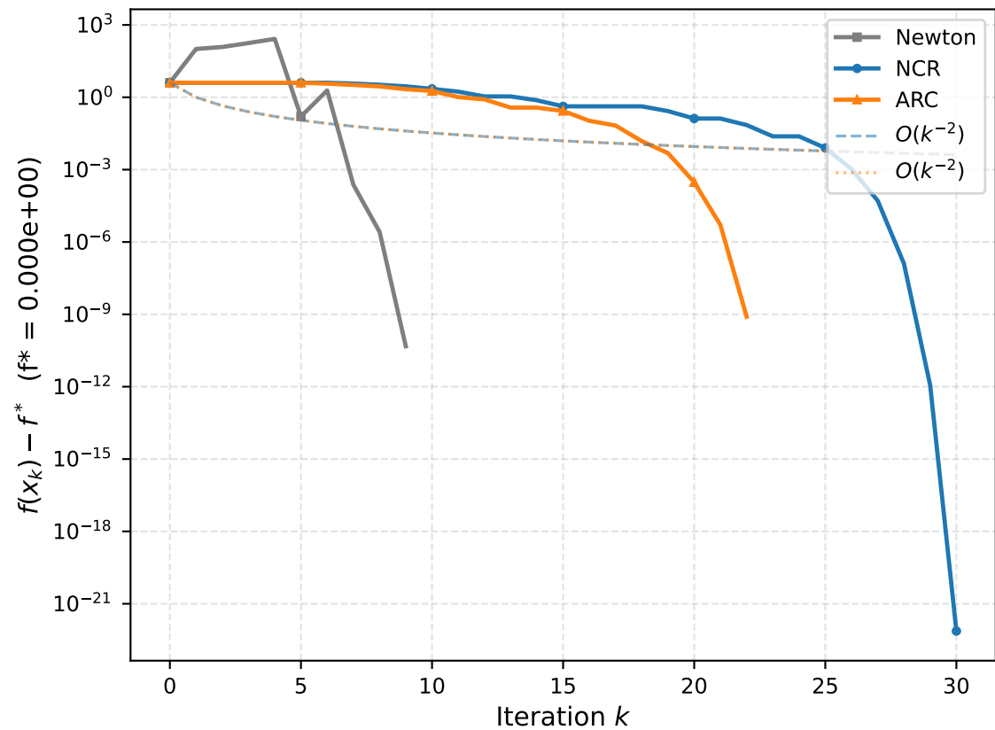
Rosenbrock (n=5) Function excess
