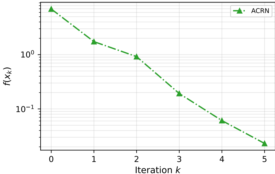
ACRN — convergence
