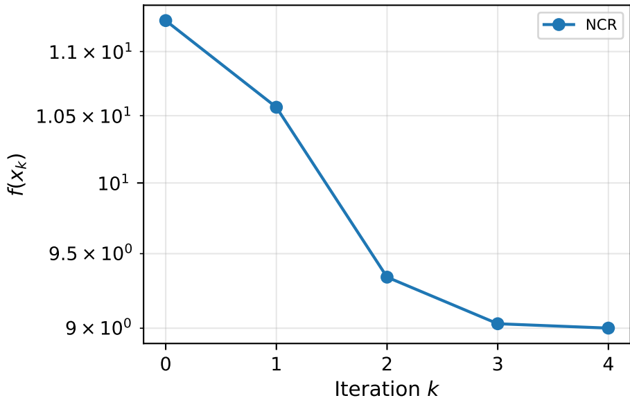
NCR — convergence
