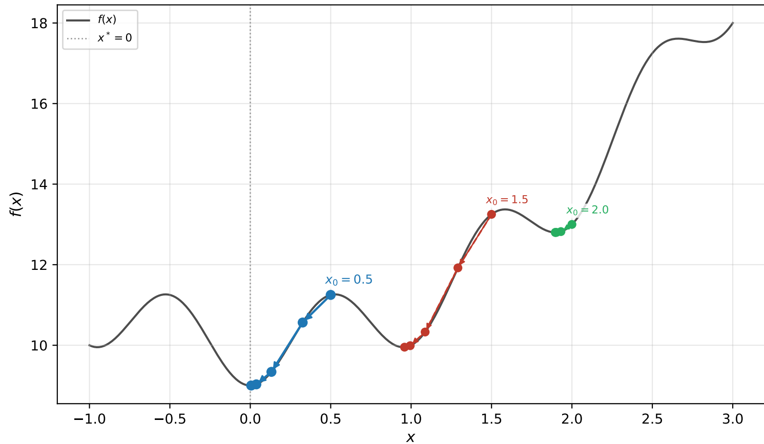
NCR — optimization paths
