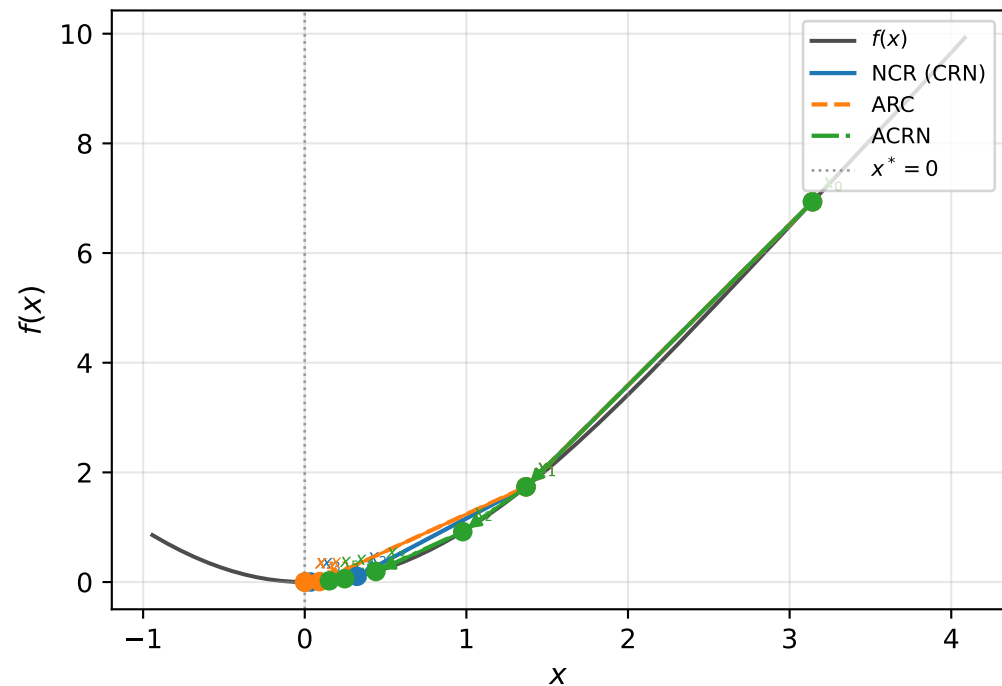
Optimization paths on f
