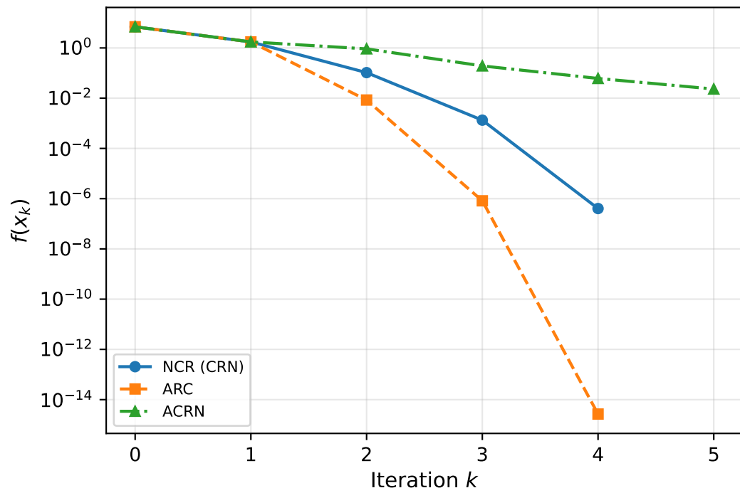
Convergence of f(x_k)
