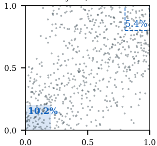
B ADNI-MEM-Amyloid Clayton, \tau=0.27
