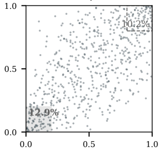
D ADNI-EF-ADNI-MEM Gaussian, \tau=0.48
