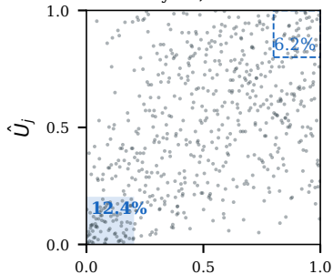
A ADNI-MEM-FDG Clayton, \tau=0.32
