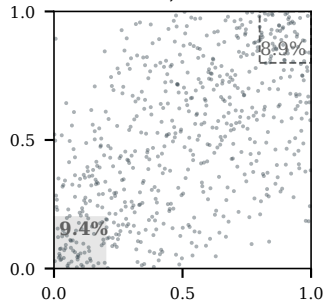
C ADNI-MEM-Hipp. vol. Frank, \tau=0.38
