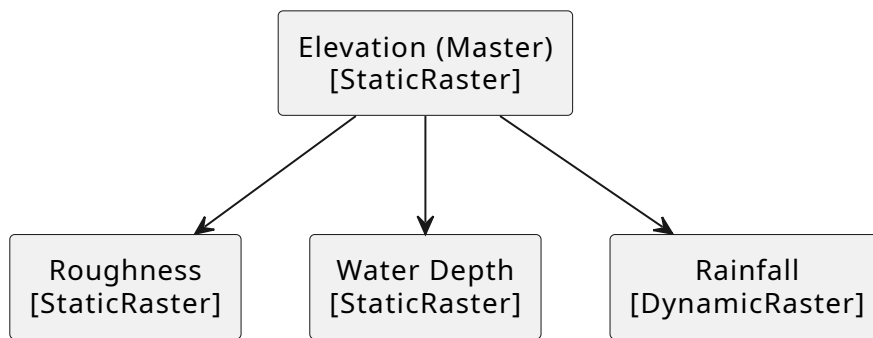
Figure 3.5: Layer Dependencies
