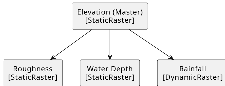
Figure 3.5: Layer Dependencies
