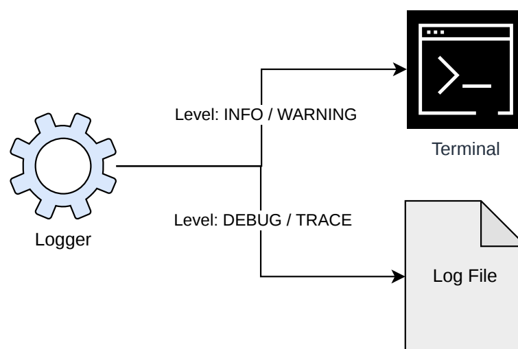
Figure 3.6: Logging Architecture
