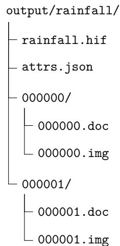
Figure 3.2: Hierarchical IDRISI Format (HIF) internal directory structure visualized as a tree topology.
