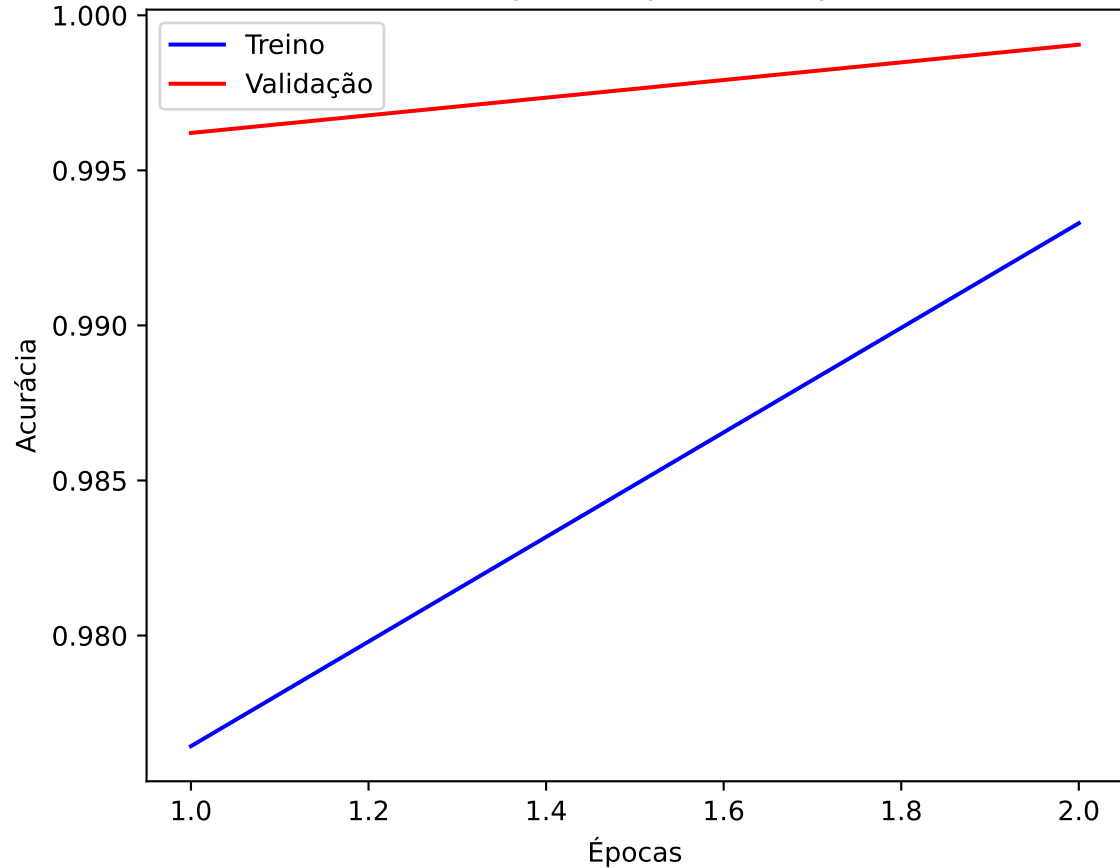
Acurácia - openai/clip-vit-base-patch16
