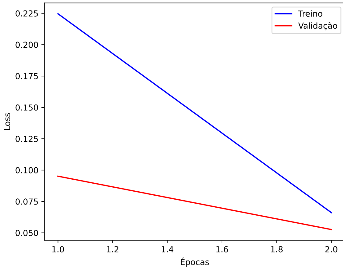
Loss - openai/clip-vit-base-patch16
