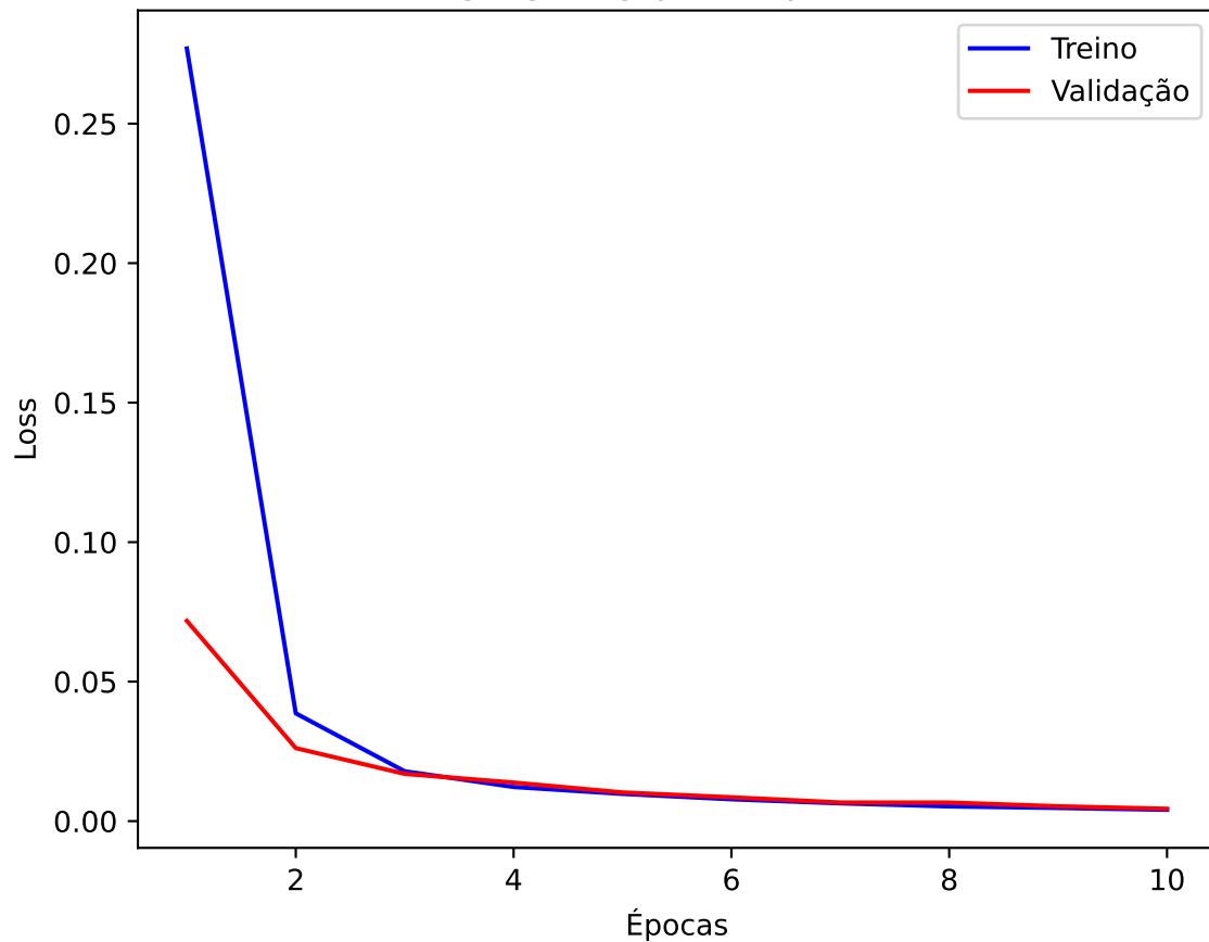
Loss - google/siglip-base-patch16-224
