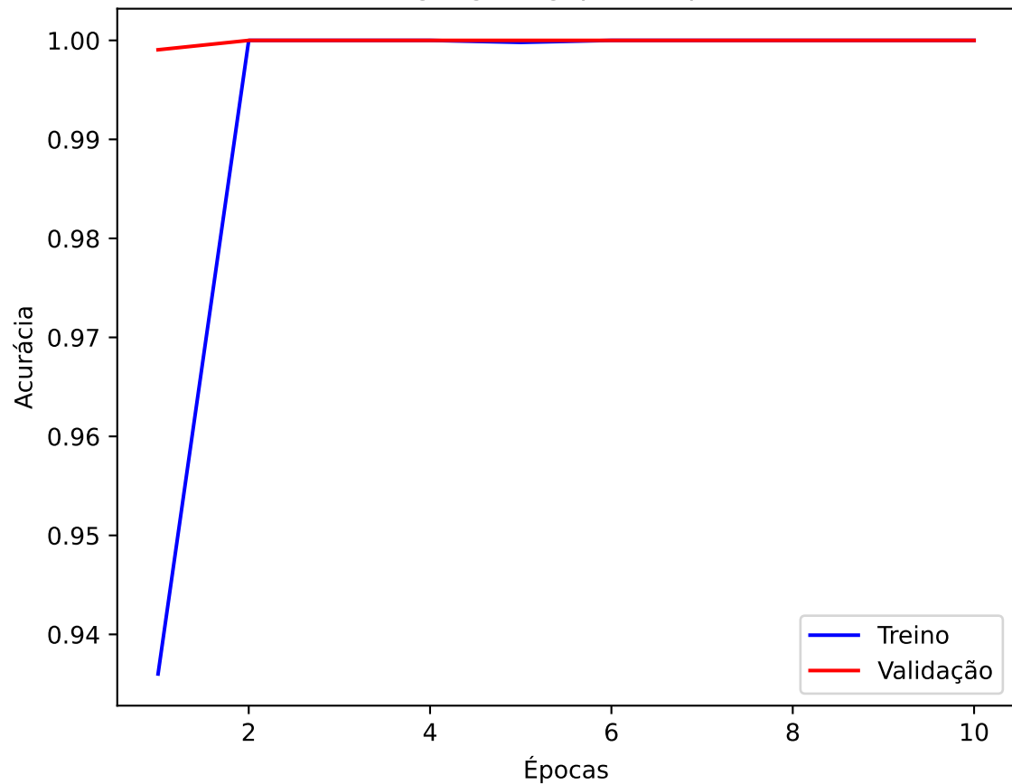
Acurácia - google/siglip-base-patch16-224
