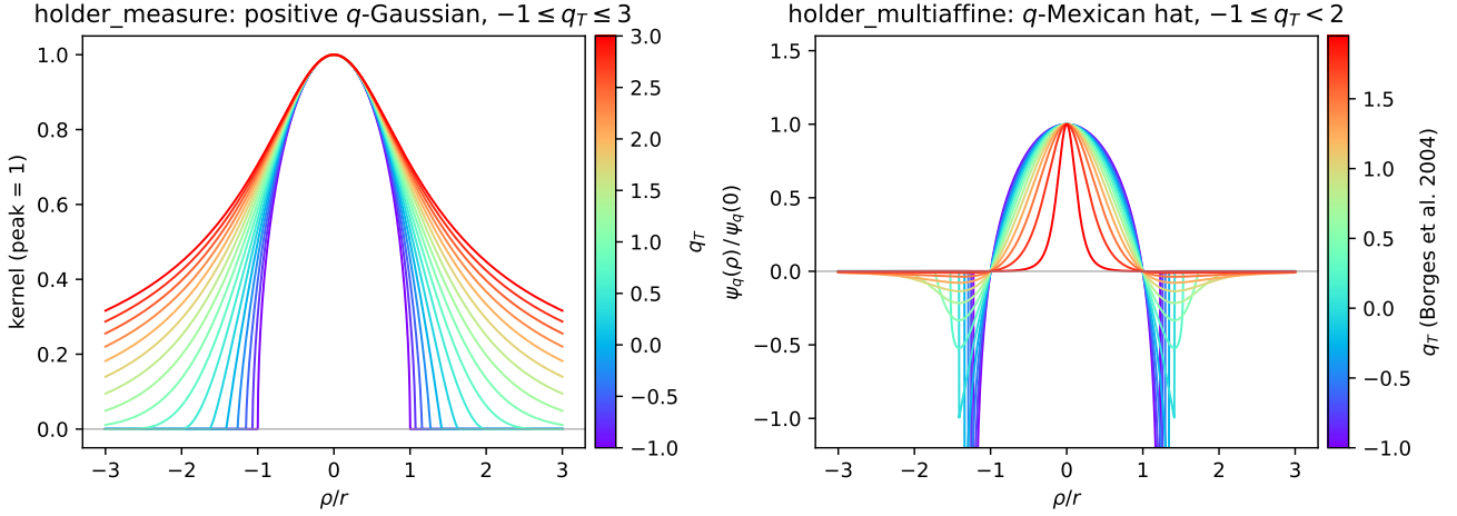
Figure 2: The q family. Left: holder_measure 's positive q-Gaussian, -1 \leq q \leq 3 (compact below q = 1 ). Right: holder_multiaffine 's q-Mexican hat (Borges et al. 2004, in 2-D), -1 \leq q < 2 ; every curve crosses zero at \rho = r , and for q < 0 the negative lobe diverges at the cutoff. Profiles scaled to 1 at the centre.
