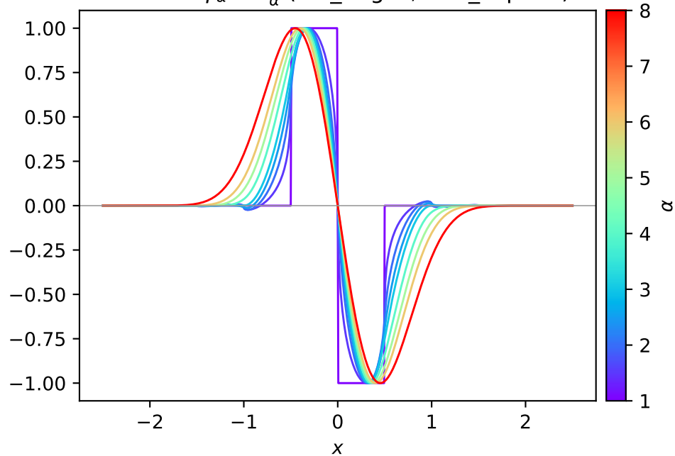
wavelet \psi_\alpha = \theta'_\alpha (mz_edges, frac_bspline)
