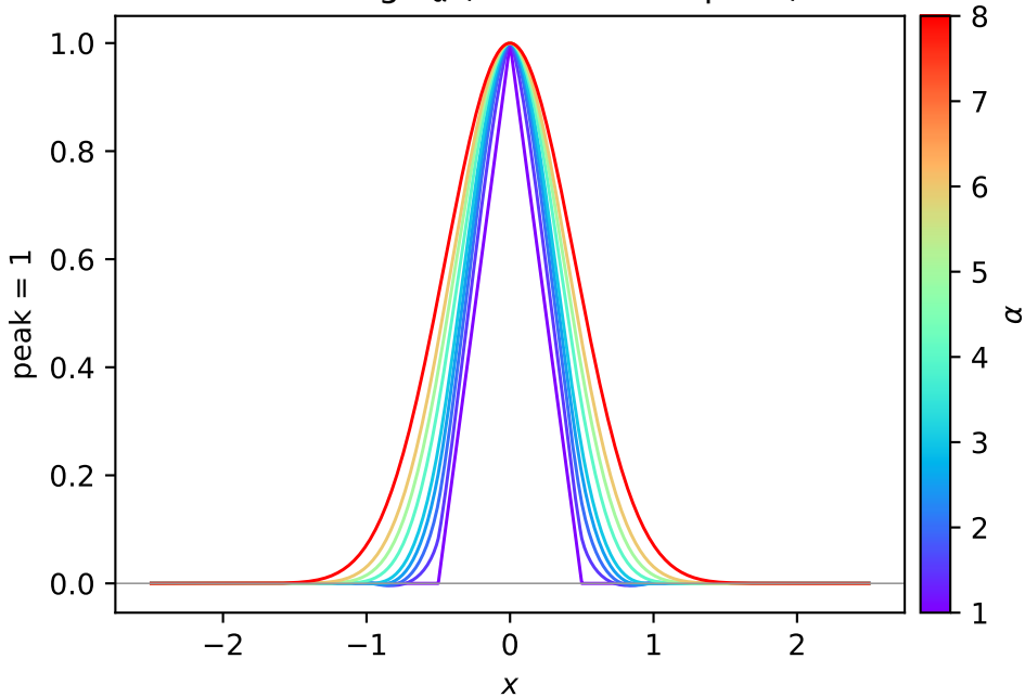
smoothing \theta_\alpha (fractional B-spline)
