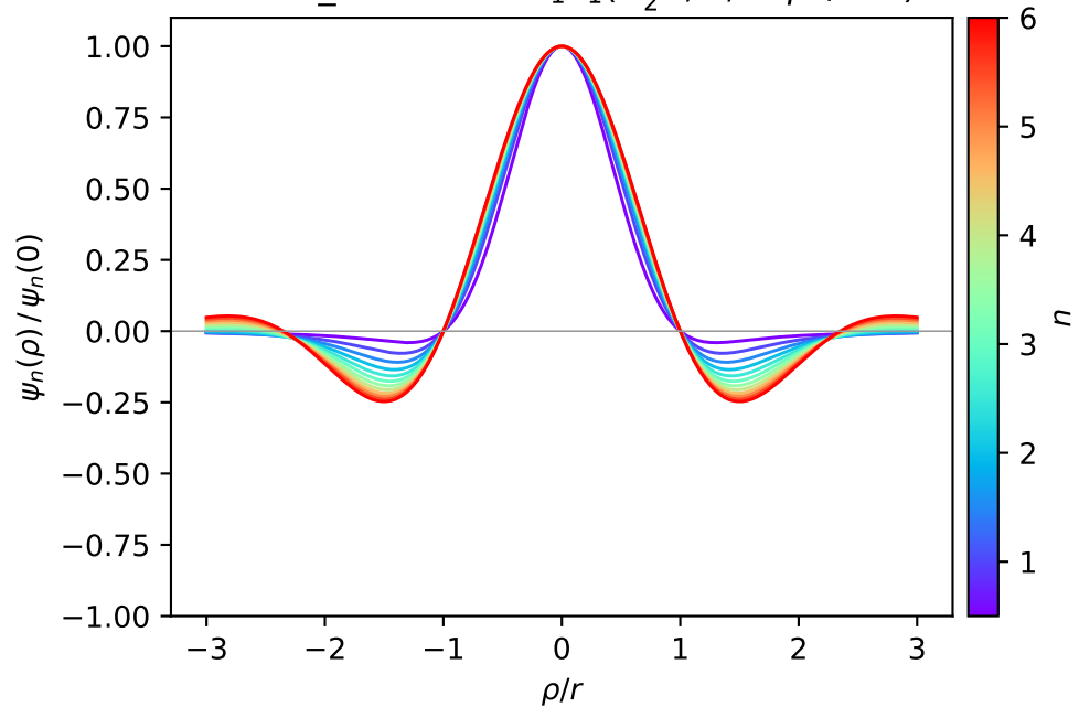
holder_multiaffine: {}_1F_1(\frac{n+2}{2}; 1; -\rho^2/2\sigma^2)
