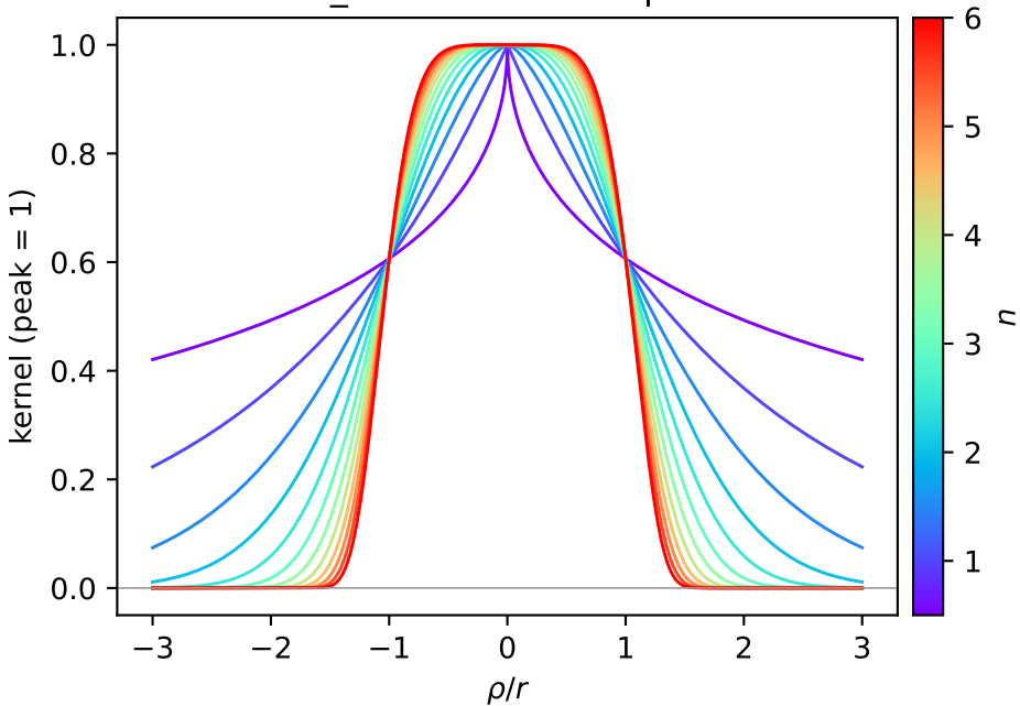
holder_measure: envelope e^{-\rho^n/2}
