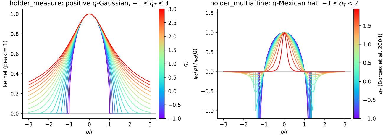
Figure 3: The q family. Left: holder_measure 's positive q-Gaussian, -1 \leq q \leq 3 (compact below q = 1 ). Right: holder_multiaffine 's q-Mexican hat (Borges et al. 2004, in 2-D), -1 \leq q < 2 ; every curve crosses zero at \rho = r , and for q < 0 the negative lobe diverges at the cutoff. Profiles scaled to 1 at the centre.
