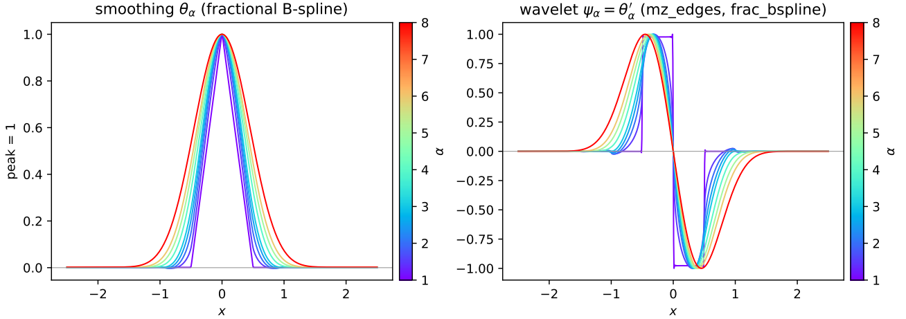
Figure 2: mz_edges, frac_bspline : the smoothing function \theta_\alpha(x) = 2\beta_*^\alpha(2x) , the symmetric fractional B-spline of degree \alpha (Unser & Blu 1999, eqs. 10–11; \hat{\beta}_*^\alpha(\omega) = |\sin(\omega/2)/(\omega/2)|^{\alpha+1} ), and the wavelet \psi_\alpha = \theta'_\alpha as \alpha varies — the analytic limit the filter cascade is pinned to (its maxima sit exactly where the classical \alpha = 3 path puts them: no causal phase). \alpha is \theta ’s Hölder degree; its approximation order is \alpha + 1 . \alpha = 1 : a triangle and a box pair; \alpha = 3 : the paper’s quadratic-spline wavelet. Only odd integer \alpha gives a compactly supported classical B-spline; other orders decay algebraically, and as \alpha \rightarrow 0 the symmetric spline is not a box but develops logarithmic peaks and oscillating tails (Unser & Blu, fig. 2). This is Mallat–Zhong’s dyadic derivative wavelet built on a fractional spline — exactly one vanishing moment ( \hat{\psi} \sim i\omega at low frequency), since maxima-are-edges is the method — not one of Unser & Blu’s fractional spline wavelet bases, which behave like fractional differentiators |\omega|^{\alpha+1} .
