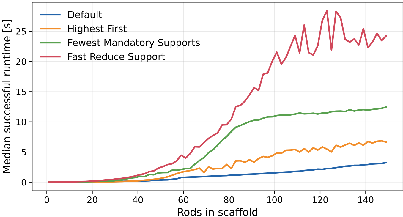
Rigidity search scaling by removal strategy
